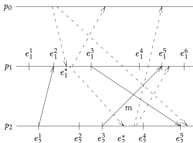
Figure 10. Application of the Chandy-Lampert Snapshot Protocol
